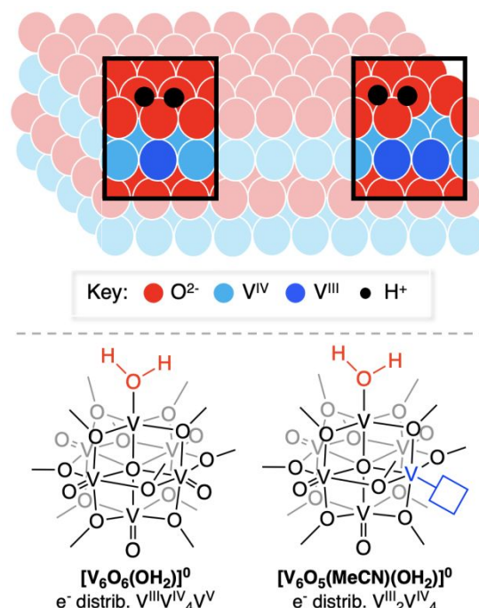
Figure 1. PCET to the surface of pristine and O-deficient metal oxide surfaces (top). 2e^-/2\text{H}^+ reduced POV-alkoxide clusters studied in this work, where V=O bond reduction occurs at the surface of a fully oxygenated vanadium oxide assembly, and one bearing a preformed O-atom vacancy to generate aquo-ligated cluster complexes.
