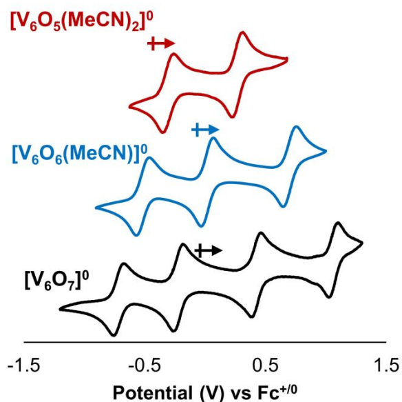
Figure 2. Cyclic voltammograms of 1 mM [\text{V}_6\text{O}_7]^0 (black), [\text{V}_6\text{O}_6(\text{MeCN})]^0 (blue), and [\text{V}_6\text{O}_5(\text{MeCN})_2]^0 (red) in DCM with 100 mM [\text{nBu}_4\text{N}][\text{PF}_6] supporting electrolyte. Arrows indicate open circuit voltages of the individual cluster complexes in their neutral charge state. Figure reproduced with permission from B. E. Petel, et al , Inorg. Chem. 2019, 58 , 10462-10471. Copyright 2019 American Chemical Society.
