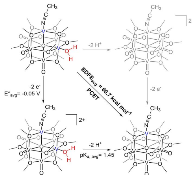
Scheme 3. Square scheme of 2e^-/2\text{H}^+ reduction of [\text{V}_6\text{O}_6(\text{OH}_2)]^{0+} to [\text{V}_6\text{O}_5(\text{MeCN})(\text{OH}_2)]^{0+} .
