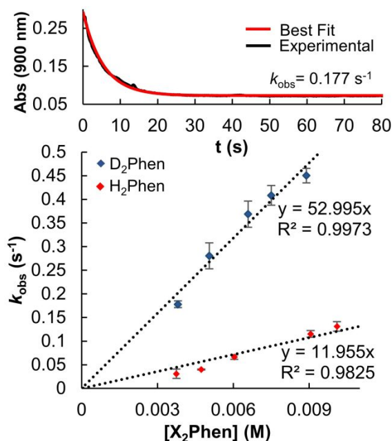
Figure 4. Determination of the observed pseudo first-order rate constant, k_{\text{obs}} , for the reduction of [\text{V}_6\text{O}_6(\text{MeCN})]^{0+} (0.75 mM) by \text{H}_2\text{Phen} (3.81 mM) in MeCN at -15 \text{ }^\circ\text{C} by monitoring absorbance at 900 nm over the reaction coordinate (top). Plot of k_{\text{obs}} as a function of [\text{X}_2\text{Phen}] , where \text{X} = \text{H}, \text{D} . Concentration of [\text{V}_6\text{O}_6(\text{MeCN})]^{0+} was held constant at 0.75 mM, and reductant concentration was varied between 3.8 and 11.5 mM. The slope of the resultant lines \times \frac{1}{2} vanadyls possible for accepting the H-atom \times \frac{1}{2} for the two chemically equivalent H-atoms transferred provides the experimentally derived second-order rate constants, k_{\text{PCET}} . Comparison of k_{\text{PCET}} for \text{H}_2\text{Phen} and \text{D}_2\text{Phen} yields a KIE of 4.4.
