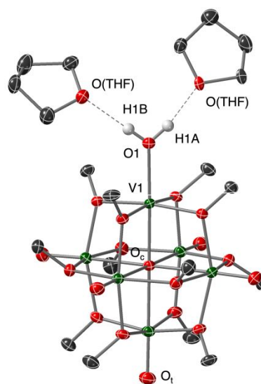
Figure 3. Molecular structure of [\text{V}_6\text{O}_6(\text{OH}_2)]^0 shown with 50% probability ellipsoids. Selected hydrogen atoms have been omitted for clarity. Key: dark green ellipsoids: V; red ellipsoids: O; dark grey ellipsoids: C; white spheres: H.
