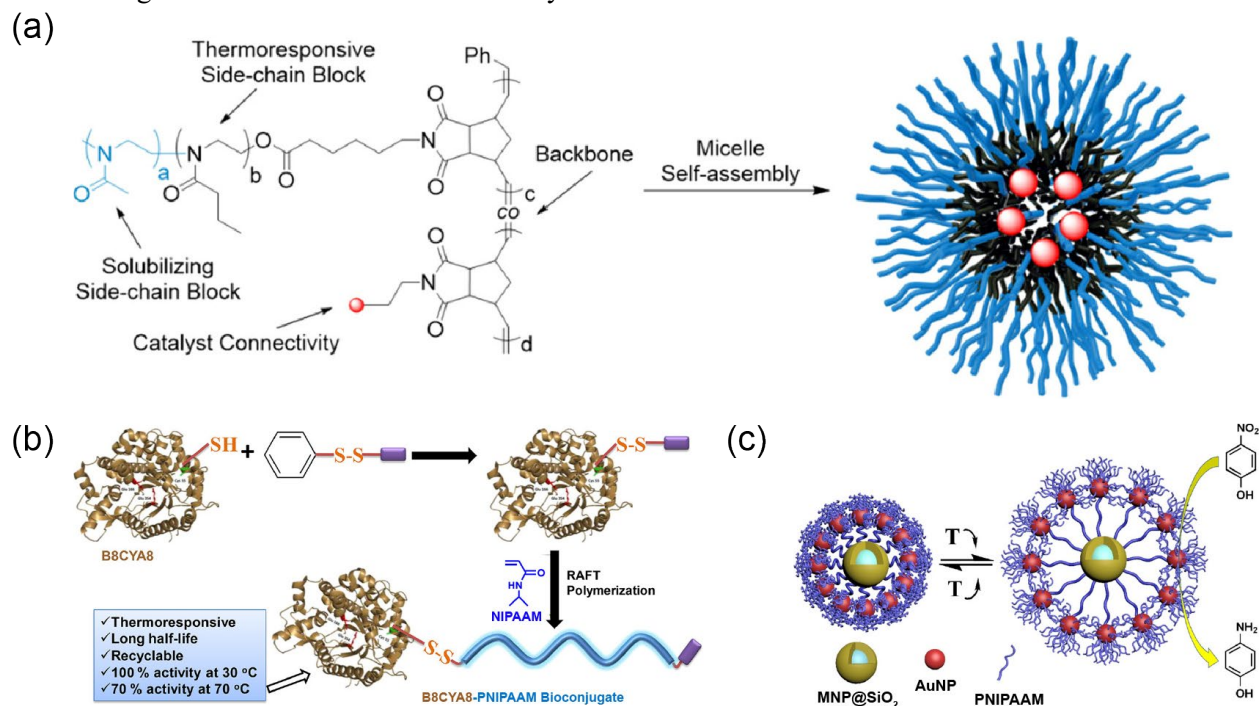
Fig. 22 Temperature-controlled catalysis (a) poly(2-oxazoline)-based bottle brush polymers applied for controlled activity and enantioselectivity of L-proline catalyst. Reproduced with permission from Ref. 96. Copyright 2021, American Chemical Society. (b) PNIPAAm conjugation to B8CYA8 b-glycosidase for modulable enzymatic activity. Reproduced with permission from Ref. 268. Copyright 2018, American Chemical Society. (c) PNIPAAm utilized as linkers and surface decorators for satellite SiO 2 -AuNPs whose substrate conversion rate was temperature-dependent. Reproduced with permission from Ref. 271. Copyright 2019, American Chemical Society.
