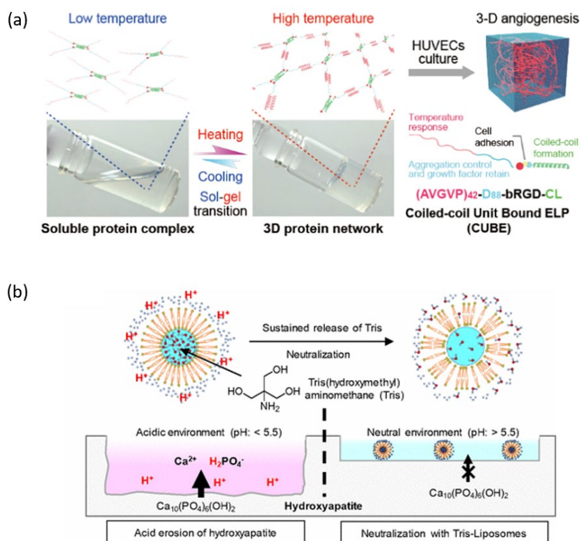
Fig. 18 (a) Genetically engineered temperature-responsive multifunctional protein hydrogels for spatiotemporal control of cellular functions. Reproduced with permission from Ref. 235. Copyright 2020 American Chemical Society. (b) Thermosensitive DPPC liposomes encapsulating alkalis successfully neutralized environmental acids for up to 3 hrs, preventing acid erosion of hydroxyapatite matrix for dental oral care. Reproduced with permission from Ref. 249. Copyright 2020 American Chemical Society.
