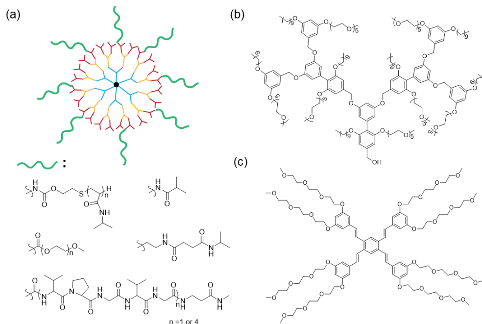
Fig. 9 Design of different types of thermoresponsive dendrimers (a) Conjugation of thermoresponsive moieties (polymer 124, 128 /small molecule 139 /peptide 127 ) to dendritic surface. Construction of dendrons with amphiphilic components containing thermoresponsive groups (b) biaryl-core facially amphiphilic G2 dendrimer 141 and (c) phenylene vinylene core G3 dendrimer. 132
