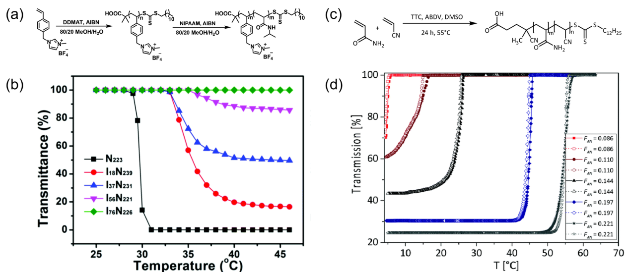
Fig. 7 Examples of effects of co-polymerization on thermoresponsive behavior. (a) Synthesis scheme of P(NIPAAAm-co-[VBMI][BF 4 ]). (b) Increasing in LCST and diminishing of thermoresponsive behavior illustrated as effects of co-polymerizing NIPAAm with a charged ionic liquid monomers. Reproduced with permission from Ref. 93. Copyright 2019, Royal Society of Chemistry. (c) Synthesis scheme of P(AAm-co-AN) (d) Elevation of UCST and more pronounced temperature sensitivity shown as impacts of co-polymerizing AAm with AN. Reproduced with permission from Ref. 95. Copyright 2017, Royal Society of Chemistry.
