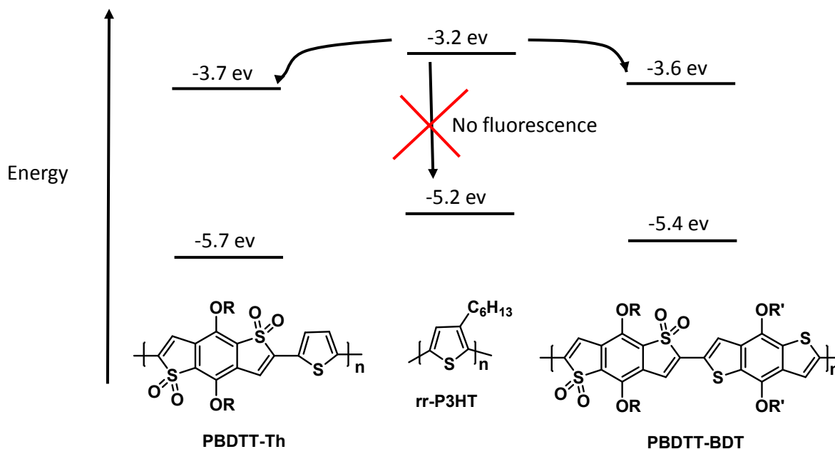
Figure 5: Illustration of the electron transfer mechanism for fluorescence quenching of rr-P3HT
