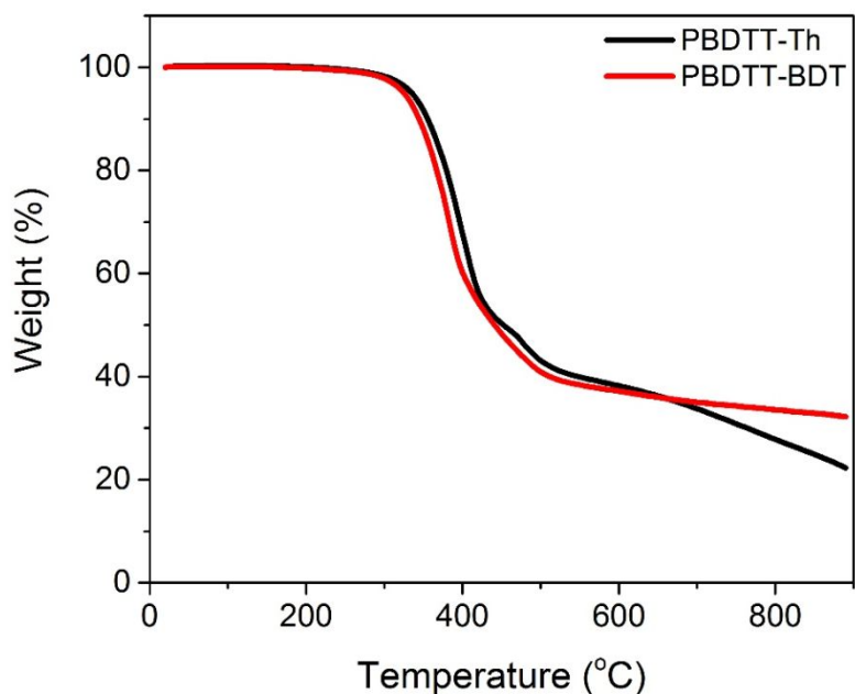
Figure 2: TGA curves of PBDTT-Th and PBDTT-BDT .
