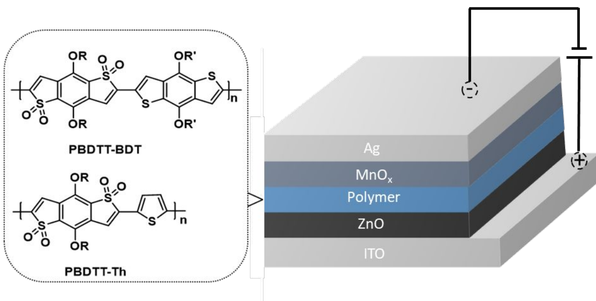
Figure 1. Device configuration for electron mobility measurements.
