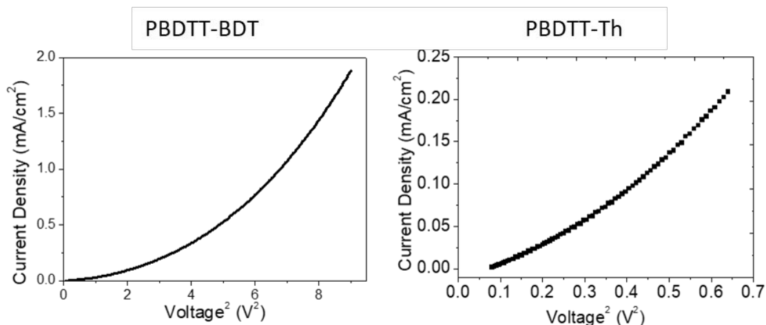
Figure 7. J-V curve of PBDTT-BDT and PBDTT-Th measured on the probe station using SCLC model.
