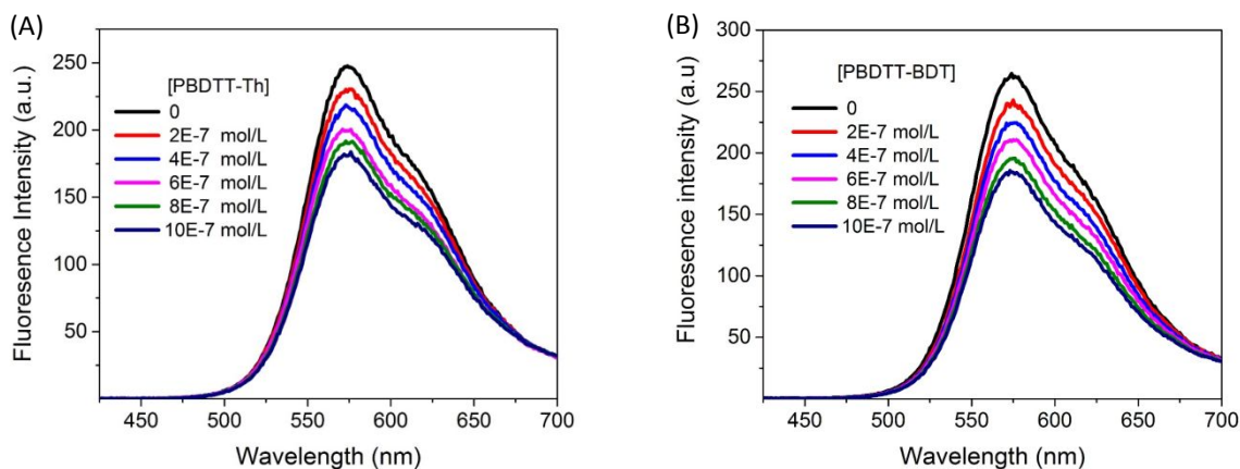
Figure 4: Fluorescence spectrum of P3HT ( 4.0 \times 10^{-7} M) in chloroform with varying concentrations of the electron acceptor (A) PBDTT-Th and (B) PBDTT-BDT .
