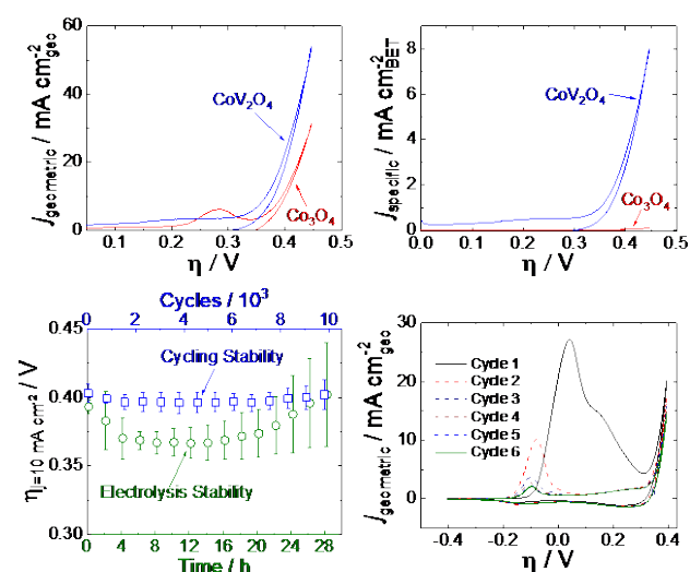
Figure 2. Cyclic RDEVs of the as-synthesized \text{CoV}_2\text{O}_4 catalyst compared to previously reported \text{Co}_3\text{O}_4 in \text{O}_2 -saturated 1 M NaOH showing (a) the current density per geometric area and (b) the specific current density per the BET surface area of the as-synthesized materials at 0.01 V/s scan rate and 1600rpm rotation rate. The RDEVs shown are the 2 nd cycle for each sample. The \text{Co}_3\text{O}_4 data is taken from Ref. 20. (c) Stability studies for the putative \text{CoV}_2\text{O}_4 during OER. The green circles are measured overpotentials at 10 \text{mA cm}^{-2} geometric ( \eta_{j=10 \text{ mA cm}^{-2}} ) during 28-h CCE measurements plotted vs the polarization time on the bottom axis. The blue squares are the \eta_{j=10 \text{ mA cm}^{-2}} values during 10,000 cycle experiments plotted vs the number of cycles on the top x-axis, and the bottom axis also reflects the time points in the cycling measurements. The \eta_{j=10 \text{ mA cm}^{-2}} values were average measurements from at least three independently-prepared samples, and the error bars represent the standard deviations. (d) The first six RDEVs measured for the as-synthesized \text{CoV}_2\text{O}_4 . There is a large pre-catalytic peak at \eta \approx 0.05 V that shifts negative and decreases in intensity in subsequent scans.
