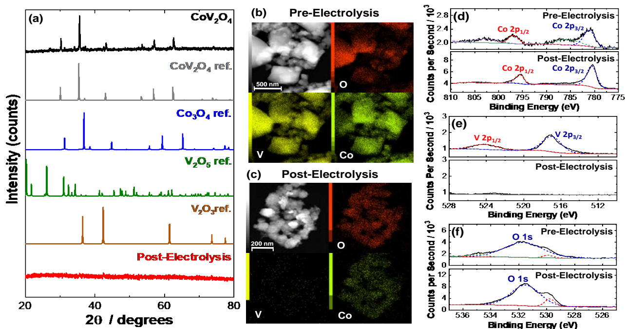
Figure 1. (a) PXRD patterns for as-synthesized \text{CoV}_2\text{O}_4 along with reference patterns for comparison. The PXRD for \text{CoV}_2\text{O}_4 after 28-h CCE under OER conditions is also included. (b) Representative TEM images and TEM-EDX maps of as-synthesized \text{CoV}_2\text{O}_4 . (c) Representative TEM images and TEM-EDX maps of \text{CoV}_2\text{O}_4 after 28-h CCE under OER conditions. (d-f) High resolution XPS spectra of \text{CoV}_2\text{O}_4 both as-synthesized and after 28-h CCE in the (d) Co 2p region, (e) V 2p region, and (f) O 1s region.
