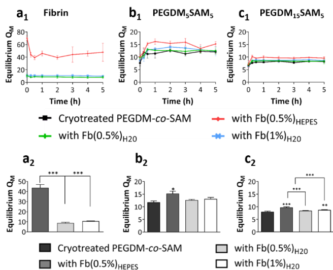
Fig. 3. Swelling characteristics of the various (a) fibrin formulations and (b, c) cryotreated PEGDM- co -SAM: Swelling kinetics for (a 1 ) fibrin formulations and across fibrin-free and fibrin-containing PEGDM- co -SAM hydrogels: (b 1 ) PEGDM 5 SAM 5 and (c 1 ) PEGDM 15 SAM 5 . Swelling mass ratio ( Q_M ) at equilibrium for (a 2 ) fibrin hydrogels and across fibrin-free and fibrin-containing PEGDM- co -SAM hydrogels: (b 2 ) PEGDM 5 SAM 5 and (c 2 ) PEGDM 15 SAM 5 . The swelling ratios Q_M at equilibrium measured on the different fibrin-containing PEGDM- co -SAM hydrogels were compared to those of fibrin-free cryotreated PEGDM- co -SAM hydrogels and to each other. Values represent mean \pm SD ( n \geq 3 ). Data were analyzed using One-way ANOVA test. * p < 0.05 , ** p < 0.01 , and *** p < 0.001 .
