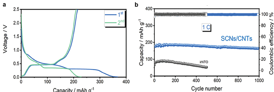
Fig. 2 (a) Typical charge/discharge profiles at 0.1C. (b) Cycling performance at 1C. Reproduced from ref. 68, licensed under Creative Commons Attribution-NonCommercial-NoDerivs Licence.
