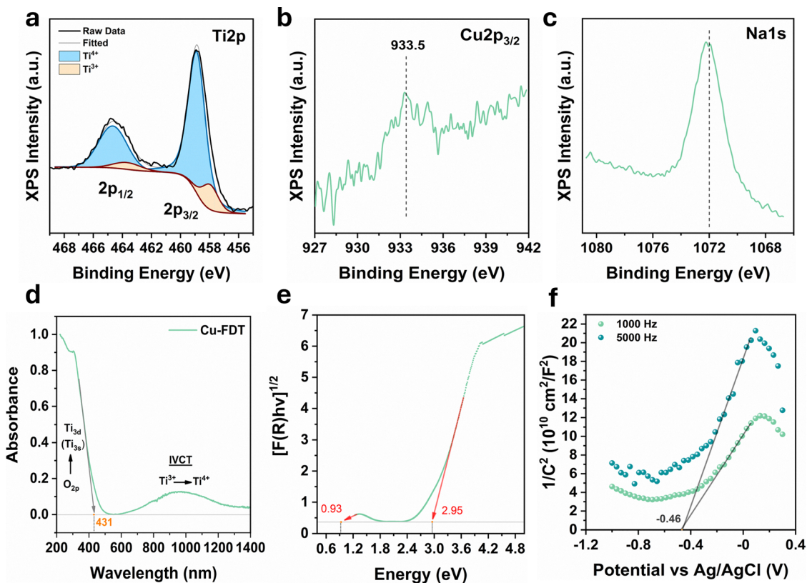
Fig. 2 (a)–(c) Fitted XPS spectra of the Ti 2p core level (a), Cu 2p 3/2 core level (b), and Na 1s core level (c) and (d) UV-DRS absorbance spectra of Cu-FDT photocatalyst, (e) Tauc plot constructed from the Kubelka–Munk transformation of Cu-FDT reflectance spectra, (f) Mott–Schottky plots obtained at 1000 and 5000 Hz.
