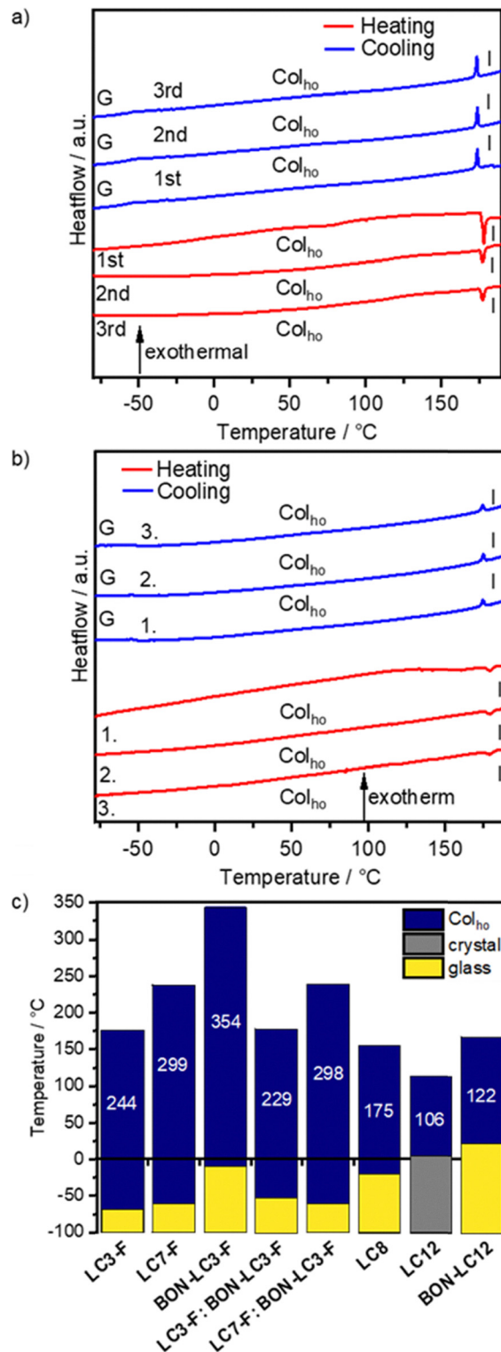
Fig. 2 (a) DSC thermogram (heating/cooling rate: 10 K min -1 ) of compound LC3-F. G = glassy state, Col ho : columnar hexagonally ordered mesophase, I = isotropic melt; (b) DSC thermogram (heating/cooling rate: 10 K min -1 ) of LC3-F doped with 1 wt% of BON-LC3-F; (c) phase ranges of the semi-perfluorinated derivatives LC3-F, LC7-F, BON-LC3-F as well as mixtures LC3-F : BON-LC3-F, LC7-F : BON-LC3-F compared with the known alkoxy derivatives LC8, LC12 and BON-LC12 respectively, determined from the second cooling cycle of the DSC measurements. Values of LC8, LC12, BON-LC12, were taken from ref. 23 and 26 for comparison.
