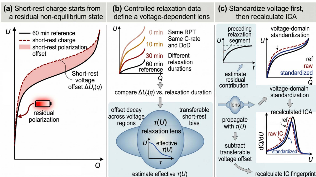
Fig. 4 Voltage-domain relaxation lens for ICA standardization: workflow of the \tau(U) -based framework. (a) Short-rest charge with residual non-equilibrium voltage offset. (b) Construction of the voltage-dependent \tau(U) relaxation lens from controlled relaxation data. (c) Voltage-domain standardization followed by ICA recalculation.
