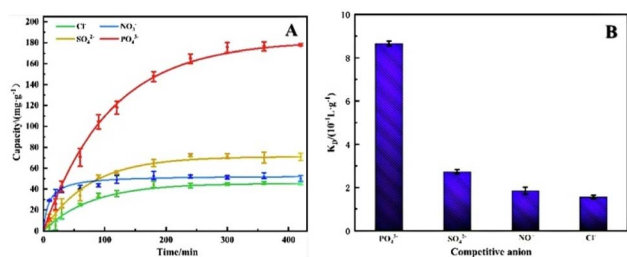
Fig. 14 (A) Competitive adsorption curve and (B) separation coefficient of PO 4 3- , SO 4 2- , NO 3 - and Cl - for NiFe-LDH/rGO hybrid films at an initial concentration of 300 ppm. Reprinted from ref. 75 with permission from Elsevier, Copyright 2022.
