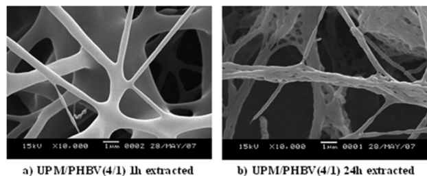
Fig. 16 Porous photocrosslinked nanofibrous structure obtained by phase separation and selective solvent extraction: SEM images of UPM/PHBV (4/1) after 1 h (a) and 24 h (b) washing step with chloroform. Figure reproduced from ref. 105 with permission from Wiley Periodicals Inc., Copyright © 2009.
