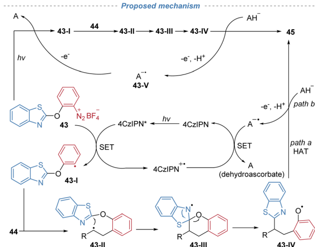
Scheme 16 Intermolecular radical difunctionalization by docking-migration of arylbenzothiazolyloether reagents.
