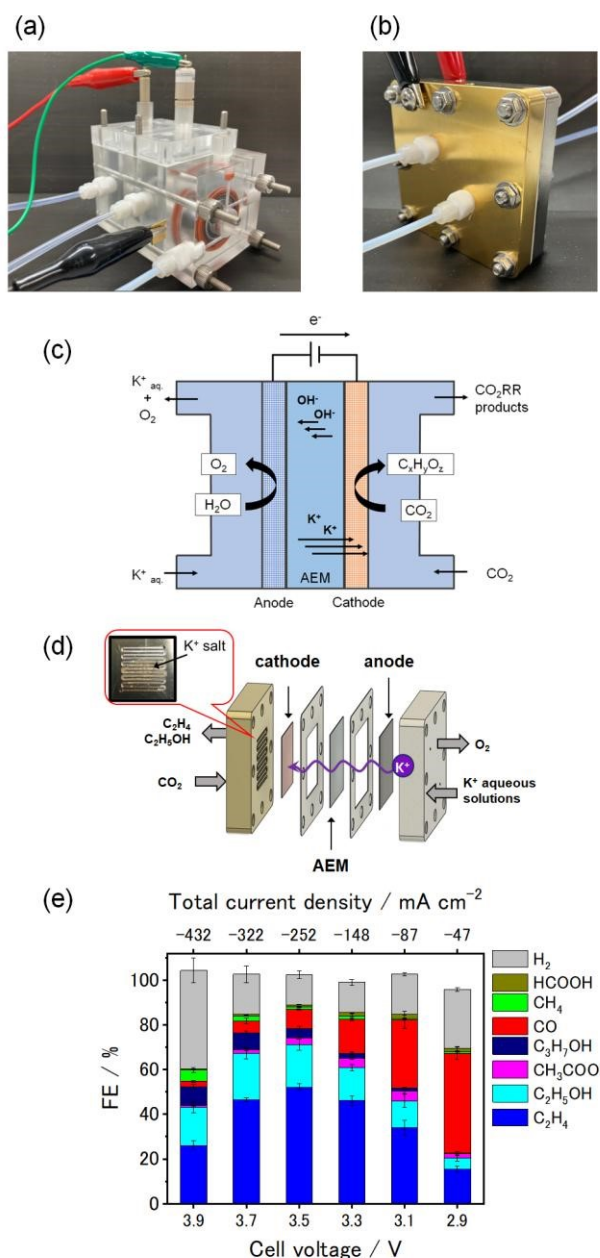
Fig. 2. Photographs of (a) the flow cell and (b) the MEA cell. (c) Cross-sectional schematic of the MEA cell. (d) Schematic of the internal structure of the MEA cell, where K + ions permeate through the AEM, leading to salt precipitation. (e) FEs of CO 2 RR products at different cell voltages using the MEA cell.
