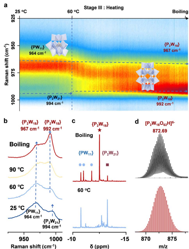
Fig. 3 (a) Stage III of heating: 2D Raman mapping (925 \text{cm}^{-1} to 1010 \text{cm}^{-1} ); (b) the corresponding Raman spectra at different temperatures; (c) ^{31}\text{P} NMR spectrum of the reaction solution at 60 ^{\circ}\text{C} and on boiling; (d) ESI-MS spectrum in negative ion mode of the solution after 24-hour reflux (the red and black lines represented simulated and experimental values, respectively).
