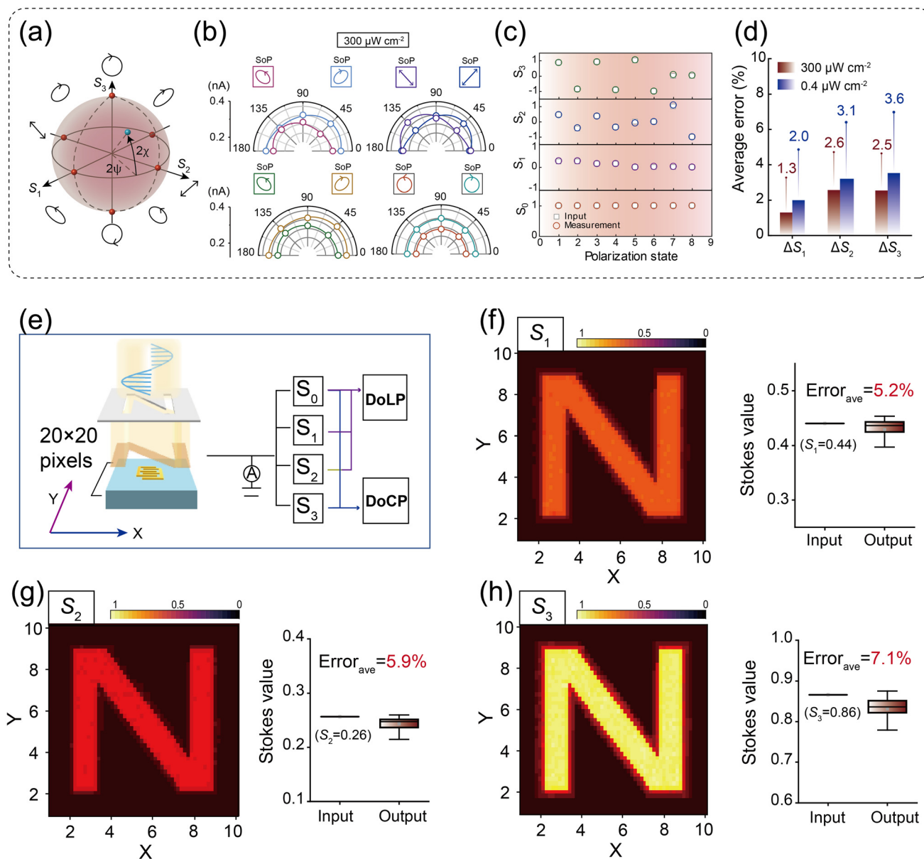
Fig. 4 (a) Poincaré sphere showing representative SoPs. (b) Measured photocurrent of the (R\text{-NEA})\text{PbI}_3 polarimeter under eight distinct input polarization states, recorded with the rotation stage set to 0^\circ, 45^\circ, 90^\circ, 135^\circ, and 180^\circ ; the incident wavelength is 396 nm with an illumination intensity of 300 \mu\text{W cm}^{-2} . (c) Detection errors for the Stokes parameters ( S_0 – S_3 ) extracted from the eight input SoPs. (d) Average detection errors for the S_1 – S_3 parameters. (e) Schematic illustration of the full-Stokes imaging test: the procedure involved transmitting modulated SoPs through an N-shaped pattern, followed by a step-by-step process to generate a 20 \times 20 pixel image array. (f–h) Full-Stokes imaging results for the S_1 – S_3 parameters and their corresponding average detection errors.
