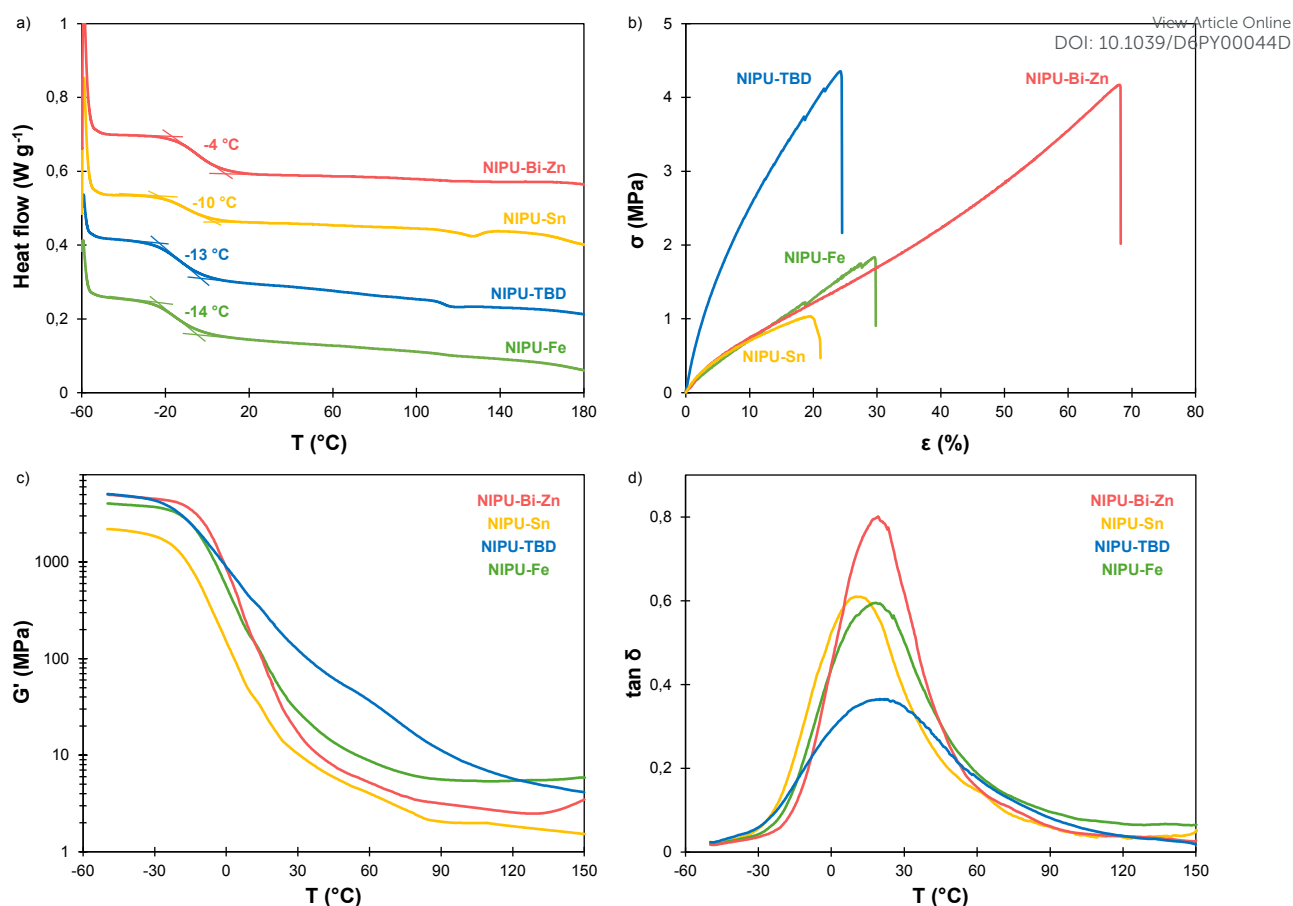
Figure 4. Characterization of the NIPU materials by (a) DSC, (b) uniaxial tensile tests, (c) storage modulus G' and (d) \tan \delta measured by DMA.
