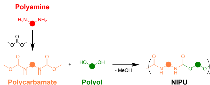
Scheme 1. Synthesis of NIPU by transurethanisation (TU).
