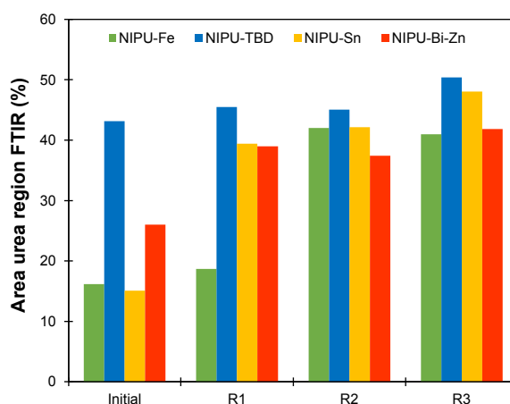
Figure 8. Proportion of the C=O stretch band in FTIR related to ureas for the different NIPU materials after several reprocessing cycles.
