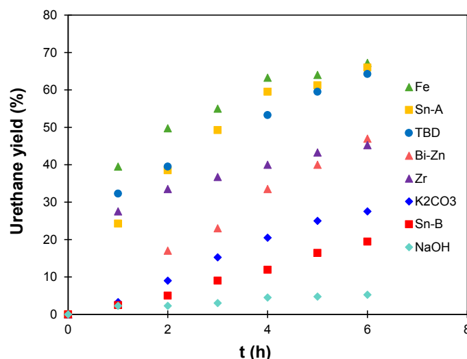
Figure 2. Kinetic study at 140 °C of the model TU reaction by 1 H NMR: yield of urethane product depending on the catalyst used.
