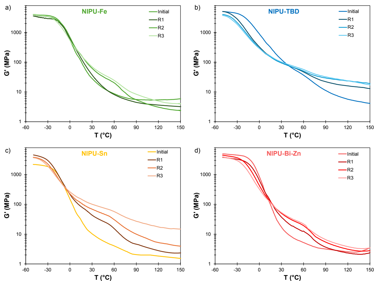
Figure 9. Storage modulus G' measured by DMA of the NIPU materials after several reprocessing cycles: (a) NIPU-Fe, (b) NIPU-TBD, (c) NIPU-Sn and (d) NIPU-Bi-Zn.
