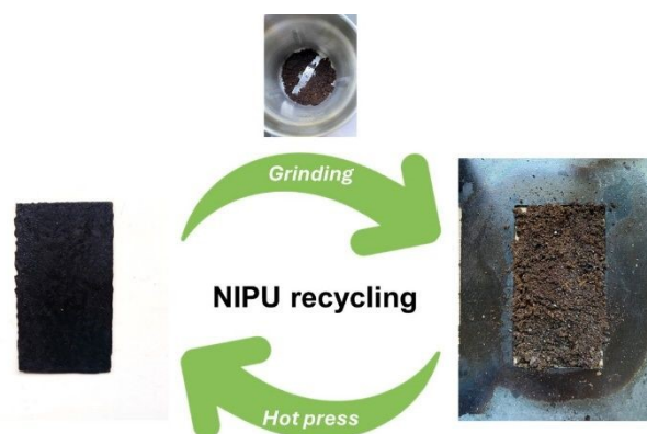
Figure 6. Recycling of NIPU materials by grinding and compression moulding.
