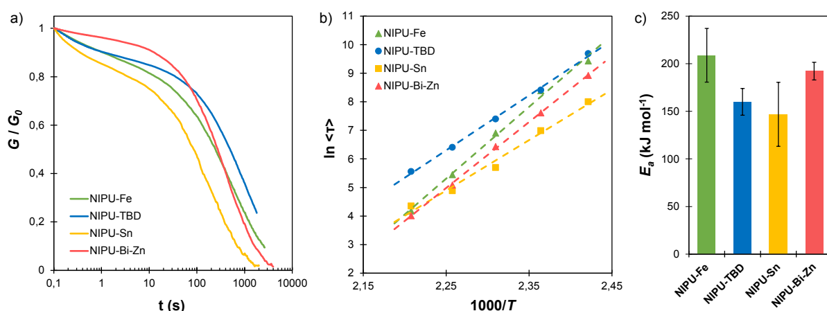
Figure 5. Results of stress relaxation experiments of the NIPU materials: (a) normalized relaxation modulus measured at 160 °C, (b) Arrhenius plot of the average relaxation times \langle \tau \rangle and (c) activation energies E_a of the bond exchange process.
