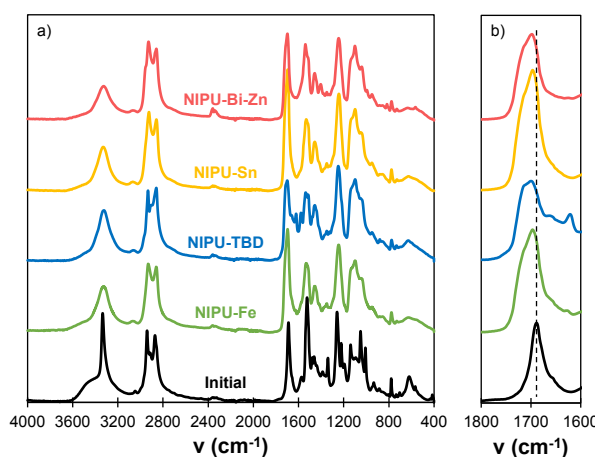
Figure 3. (a) FTIR spectra of the initial reactant mixture before polymerization and the resulting NIPU materials prepared with various catalysts. (b) Detail of the C=O stretch region.
