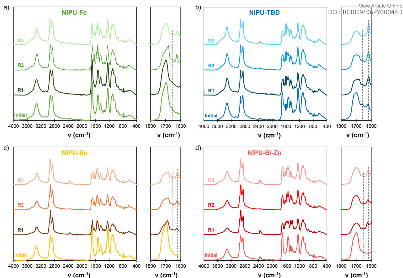
Figure 7. FTIR spectra of the NIPU materials after several reprocessing cycles: (a) NIPU-Fe, (b) NIPU-TBD, (c) NIPU-Sn and (d) NIPU-Bi-Zn.
