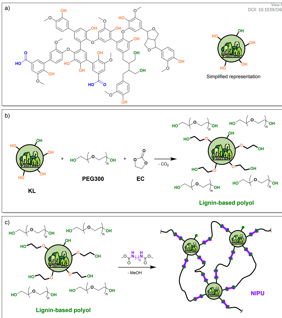
Figure 1. (a) Representative structure of KL, (b) scheme of lignin-based polyol synthesis with EC and (c) scheme of NIPU synthesis from lignin-based polyol and HMDI.
