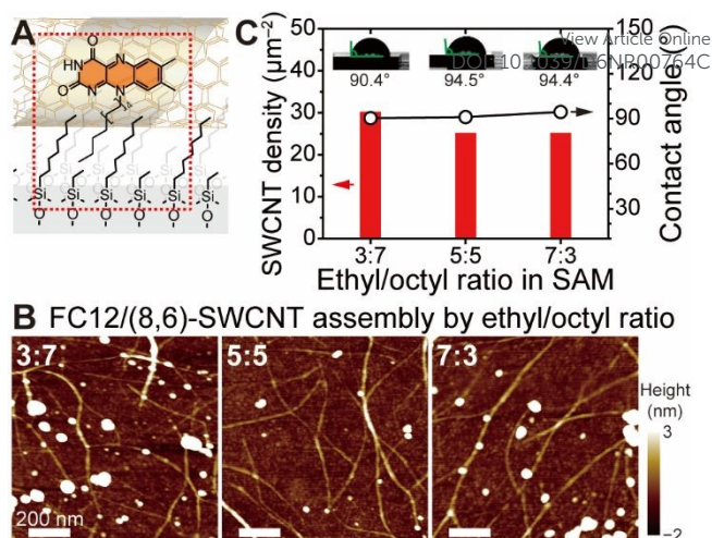
Fig. 3 Maximized FC12/(8,6)-SWCNT random network film assembled on varying tandem alkyl SAMs. (A) Schematic for FC12/(8,6)-SWCNT assembled on an ethyl:octyl tandem SAM. (B) AFM images of the assembled FC12/(8,6)-SWCNT random networks according to ethyl/octyl ratio in SAMs. Scale bar: 200 nm. (C) SWCNT density and water contact angle according to ethyl/octyl ratio of SAM.
