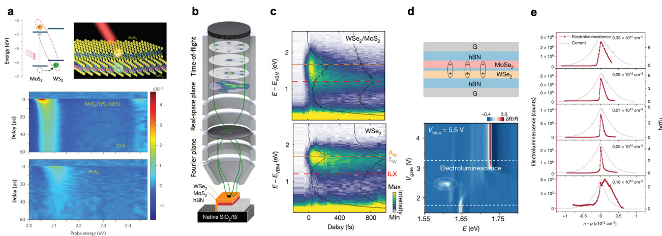
Fig. 4 (a) (Top) Schematic diagram of interlayer exciton formation in \text{MoS}_2/\text{WS}_2 heterostructure with type II band alignment. Transient absorption spectra versus probe energy at 77 K in (middle) \text{MoS}_2/\text{WS}_2 heterostructure and (bottom) \text{MoS}_2 monolayer upon \text{MoS}_2 A-exciton excitation; reproduced from ref. 57 with permission from Springer Nature, copyright 2014. (b) Schematic of femtosecond momentum microscopy. (c) Pump–probe delay dependent evolution of the momentum-integrated energy-distribution curves for (top) \text{WSe}_2/\text{MoS}_2 heterostructures and (bottom) isolated \text{WSe}_2 ; reproduced from ref. 67 with permission from Springer Nature, copyright 2022. (d) Schematic of \text{MoSe}_2/\text{WSe}_2 heterobilayer devices with electron–hole double-layer structures. (Top) Differential reflection, \delta R/R , versus photon energy E and gate voltage V_{\text{gate}} . Electroluminescence from the tunnel junction is visible in the circled bright spot. (e) (Left axis) Electroluminescence intensity and (right axis) tunnelling current versus electron–hole density imbalance for variable total densities. A threshold behavior with a cusp-shaped peak emerges, indicative of the formation of exciton condensation; reproduced from ref. 68 with permission from Springer Nature, copyright 2019.
