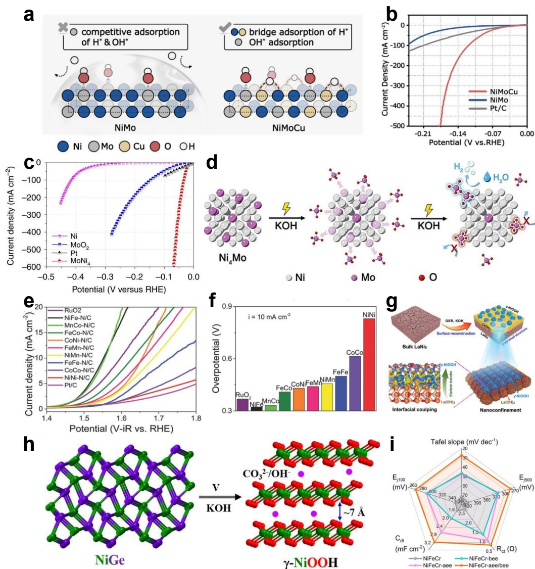
Fig. 8 (a) Schematic illustration of the competitive adsorption of \text{OH}^* and \text{H}^* on the Mo site of the \text{NiMo} alloy, and the separated adsorption of \text{OH}^* and \text{H}^* on the Mo site and Ni-Cu dual site of the \text{NiMoCu} alloy. (b) Linear sweep voltammetry (LSV) curves of \text{NiMoCu} , \text{NiMo} , and \text{Pt/C} . Reproduced from ref. 175 with permission from Wiley-VCH, copyright 2025. (c) Polarization curves of the \text{MoNi}_4 electrocatalyst supported on \text{MoO}_2 cuboids, compared with pure Ni nanosheets and \text{MoO}_2 cuboids deposited on Ni foam. Reproduced from ref. 176 with permission from Springer Nature, copyright 2017. (d) Schematic illustration of the role of Mo in the \text{Ni}_4\text{Mo} alloy during alkaline HER. Reproduced from ref. 181 with permission from John Wiley and Sons Ltd, copyright 2021. (e) LSV polarization curves for different binary alloy samples, \text{Pt/C} , and \text{RuO}_2 in \text{O}_2 saturated 0.1 M \text{KOH} , (f) overpotential at a current density of 10 \text{ mA cm}^{-2} . Reproduced from ref. 198 with permission from Wiley-VCH, copyright 2017. (g) Schematic illustration of how La enhances the OER performance of the \text{LaNi}_5 precatalyst. Reproduced from ref. 199 with permission from Wiley-Blackwell, copyright 2023. (h) Crystal structures of \text{NiGe} and electrochemically formed \gamma\text{-NiOOH} . When a potential is applied in an alkaline \text{KOH} electrolyte, Ge is fully dissolved, resulting in the formation of \gamma\text{-NiOOH} . Reproduced from ref. 200 with permission from John Wiley and Sons Ltd, copyright 2021. (i) Radar graph comparing the overpotentials (at 100 and 500 \text{mA cm}^{-2} ), Tafel slope, charge transfer
