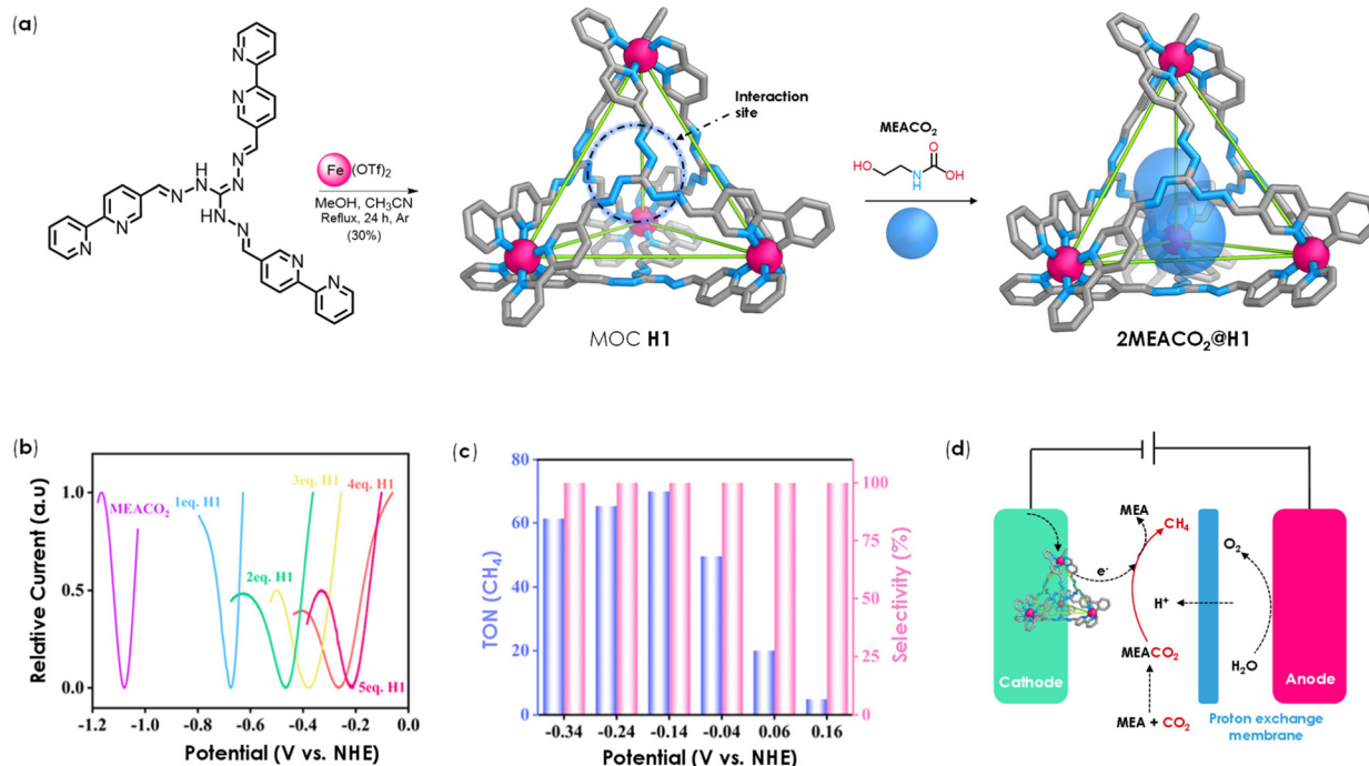
Fig. 5 (a) Schematic process of self-assembly to produce H1 and the formation of the host–guest 2\text{MEACO}_2@H1 adduct. (b) Square wave voltammetry (SWV) of the systems containing \text{MEACO}_2 (0.1 mM) at different concentrations of H1. (c) Relationship between TON and selectivity for the electrocatalytic reduction of \text{CO}_2 to \text{CH}_4 by H1 at different controlled potentials. (d) Schematic diagram of the cavity-mediated mechanism for the conversion of \text{MEACO}_2 into \text{CH}_4 within tetrahedron H1. Parts (b–d) adapted from ref. 60, https://doi.org/10.1039/d5qi00756a . Copyright 2025, The Royal Society of Chemistry.
