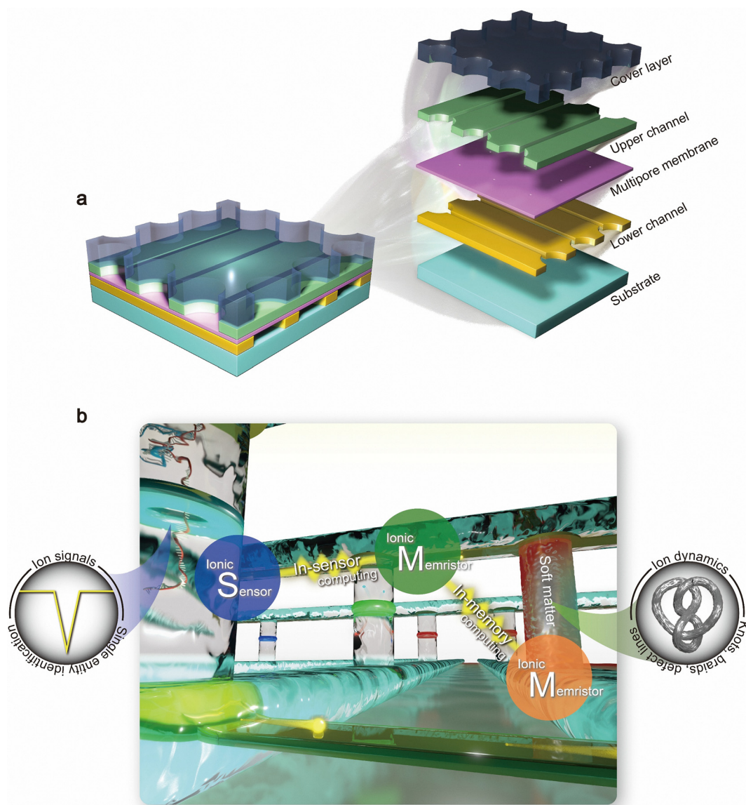
Fig. 12 Crossbar nanopore junction system. (a) Schematic of a crossbar architecture in which row and column fluidic channels are patterned on opposite sides of a multipore membrane, so that each channel intersection defines an individually addressable nanopore junction. Selecting a specific row-column pair localizes the applied bias and ionic flux to the corresponding junction, enabling dense, addressable ionic memristor arrays in a layout analogous to crossbar RRAM. Expanded view of the stacked implementation (cover layer, upper channel layer, multipore membrane, lower channel layer, and substrate) illustrates a manufacturable route to scaling nanopore-junction devices with simplified interconnect routing and on-chip integration. (b) Conceptual nanopore-junction architecture for in-sensor and in-memory computing each addressable junction senses ionic events while nearby adaptive conductance stores local context, enabling in-sensor classification and in-memory computing with analogue ionic weights.
