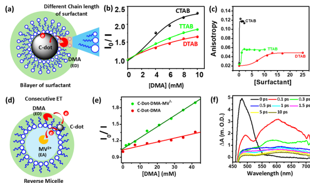
Fig. 4 (a) Surfactant chain length controls the ET process in cationic surfactant (CTAB, TTAB, and DTAB) bilayer-protected C-dots. (b) Extent of C-dot quenching by DMA as a function of the chain length of the surfactant coated around C-dots in aqueous medium. (c) Steady state anisotropy of C-dots upon interaction with cationic surfactants with different chain lengths; adapted from ref. 62 with permission from the American Chemical Society, copyright 2025. (d) Successive ET processes in encapsulated C-dots and DMA (donor, in a nonpolar environment) and MV^{2+} (acceptor, in a polar environment). (e) Relative quenching of C-dots by DMA in the presence and absence of MV^{2+} . (f) TA spectra of DMA-CNP- MV^{2+} in AOT/hexane reverse micelles following a 400 nm laser pulse excitation; adapted from ref. 75 with permission from the American Chemical Society, copyright 2025.
