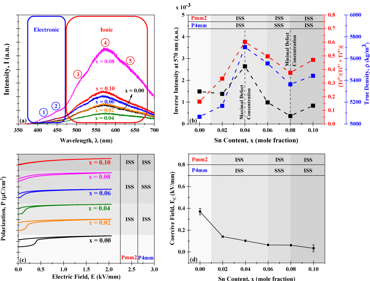
Fig. 4 (a) Photoluminescence spectra, (b) variation in inverse 570 nm intensity, true density and \frac{[\text{Ti}^{3+}]}{[\text{Ti}^{3+}] + [\text{Ti}^{4+}]} as a function of \text{Sn}^{4+} doping level, (c) unipolar polarization curves (vertically offset) measured at 2.0 \text{ kV mm}^{-1} , and (d) variation in coercive field, E_C as a function of \text{Sn}^{4+} doping level for (\text{Ba}_{0.85}\text{Ca}_{0.15})([\text{Ti}_{0.92-x}\text{Sn}_x]\text{Zr}_{0.08})\text{O}_3 ( x = 0.00-0.10 ).
