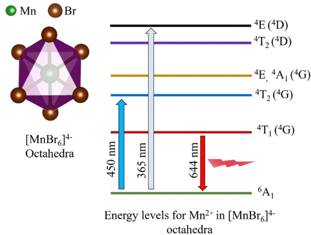
Fig. 8 Energy level diagram of octahedrally coordinated Mn 2+ ions in CsMnBr 3 , depicting d–d transitions and the photoluminescence pathway for red emission ( \sim 644 nm).
