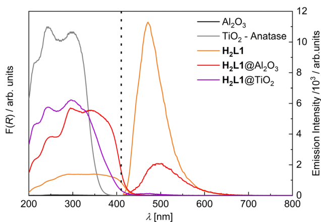
Fig. 4 Diffuse reflectance spectra (Kubelka–Munk analysis, left) and photoluminescence spectra (right) of bulk H 2 L1 , the neat substrates \text{TiO}_2 and \text{Al}_2\text{O}_3 , and the hybrid materials. Dashed line represents the excitation wavelength of 410 nm for the PL experiments.
