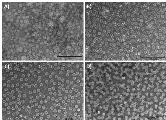
Fig. 2 TEM micrographs of BMV in different solvents. (A) Micrograph of BMV viruses in 30% ethanol. (B) Micrograph of BMV viruses in 30% isopropanol. (C) Micrograph of BMV viruses in 30% methanol. (D) Micrograph of BMV viruses in 50% DMSO. Magnifications 40 k \times , scale 200 nm.
