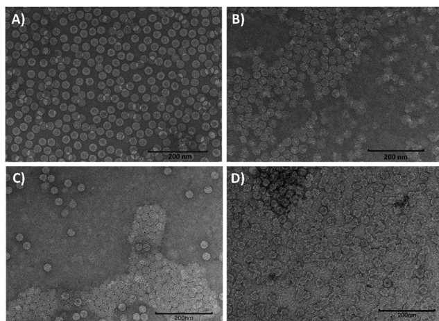
Fig. 3 TEM micrographs of CCMV in different solvents. (A) Micrograph of CCMV viruses in 50% ethanol. (B) Micrograph of CCMV viruses in 30% isopropanol. (C) Micrograph of CCMV viruses in 30% methanol. (D) Micrograph of CCMV viruses in 50% DMSO, magnifications 40 k \times , scale 200 nm.
