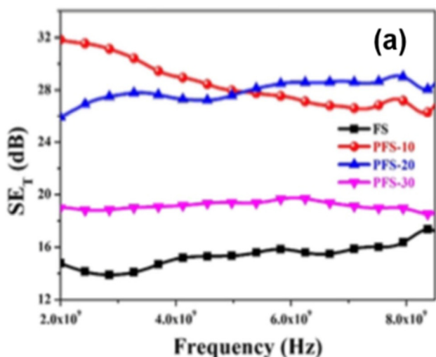
Fig. 21 (a) Plot of frequency versus SE_T of \text{Fe}_3\text{O}_4@(\text{SiO}_2)_x@(\text{PPy})_y (PFS) nanocomposites (Pyrrole/ \text{Fe}_3\text{O}_4@(\text{SiO}_2) (PS) = 9 : 1, 8 : 2, and 7 : 3) with the aniline monomer under identical reaction conditions and procedures, and the samples were designated as (PFS-10, PFS-20, and PFS-30, respectively), and (b) tuning of shells in trilaminar \text{Fe}_3\text{O}_4@(\text{SiO}_2)_x@(\text{PPy})_y and \text{Fe}_3\text{O}_4@(\text{C})_x@(\text{PANI})_y core@shell nanocomposites in controlling electromagnetic interference through switching of the shielding mechanism. 384 Reproduced with permission from ACS.
