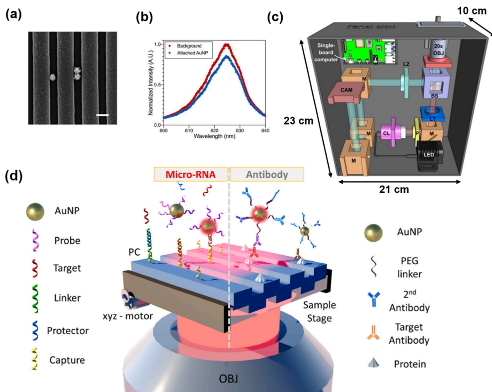
Fig. 12 Photonic resonator absorption microscopy for point-of-care biosensing. (a) Principles of PRAM operation using photonic crystals (SEM scale bar 200 nm) and (b) nanoparticles coupled with a red LED. Reproduced with permission from ref. 427. Copyright 2022, Elsevier. (c) Miniaturized PRAM-mini setup and dimensions for point-of-care detection, adapted from Khemtonglang et al. Reproduced with permission from ref. 424. Copyright 2024, Optica Publishing Group. (d) PRAM assays for testing microRNA and proteins, adapted from Liu et al. Reproduced with permission from ref. 423. Copyright 2024, Elsevier.
