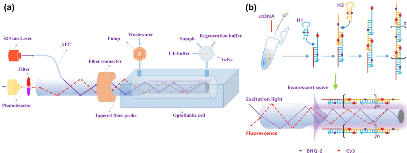
Fig. 11 Design and operation of the HCR-LOFD system. (a) Schematic of the lab-on-fiber platform, comprising a 520 nm laser, asymmetric Y-branch fiber coupler (AFC), optofluidic unit, and photodetector. (b) Target ctDNA hybridizes with hairpin H1, triggering HCR with hairpin H2 to form nicked DNA helices. This structural change separates fluorophore-quencher pairs, reducing FRET and restoring Cy3 fluorescence within the evanescent field. Emitted fluorescence is coupled back through the AFC to a photodiode for end-point or real-time detection. The system enables quantitative ctDNA detection within 6 min at room temperature, directly from diluted whole blood. 414 Reproduced with permission from ref. 414. Copyright 2023, Elsevier.
