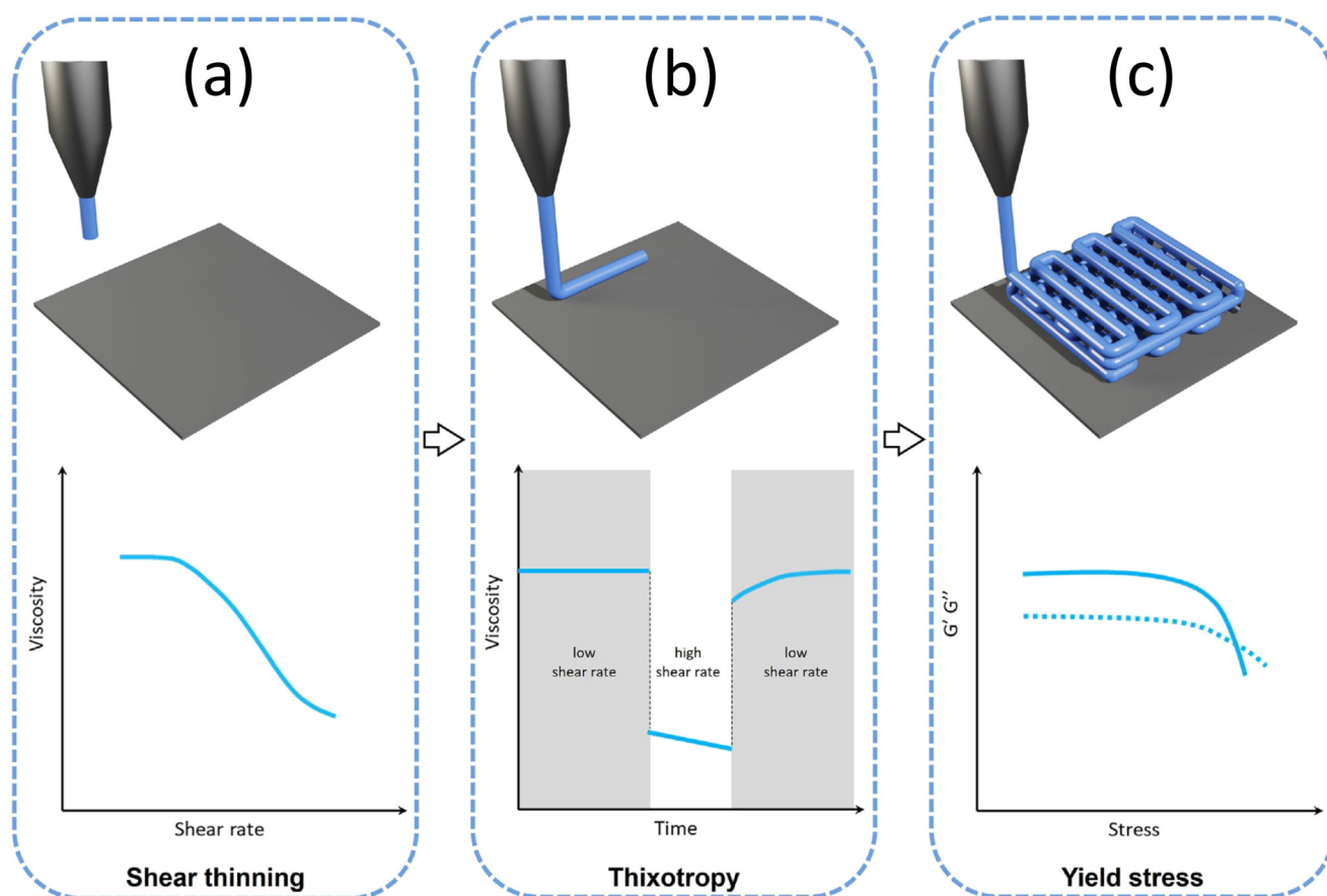
Fig. 11 Schematic description of direct ink printing, highlighting the important role of ink rheology in different stages of printing. (a) Favorable shear-thinning effect on the ink flow-ability at the early stage of printing. (b) Significance of ink thixotropy (less thixotropic is more favorable) at the printing stage when the ink settles on the substrate. (c) Yield stress and viscoelasticity effects on the quality of the printed structure. Adapted from ref. 161.
