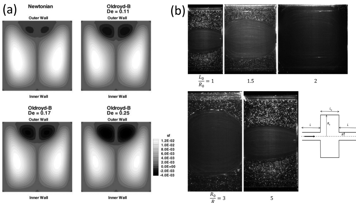
Fig. 10 (a) Effect of fluid viscoelasticity on Dean vortices at three Deborah numbers ( De = 0.11, 0.17 , and 0.25 ), with the Dean number fixed ( Dn = 150 ). Results are compared with the Newtonian-fluid counterpart. Adapted from ref. 157 with permission from Elsevier, copyright 2009. (b) Effect of geometry on the flow of a yield-stress fluid (Carbopol gel) in an expansion-contraction chamber. In each case, the flow is from left to right, and the illuminated regions at the bottom and top indicate unyielded (stagnant) zones, whereas the flow is yielded in the central region. Adapted from ref. 159 with permission from Elsevier, copyright 2007.
