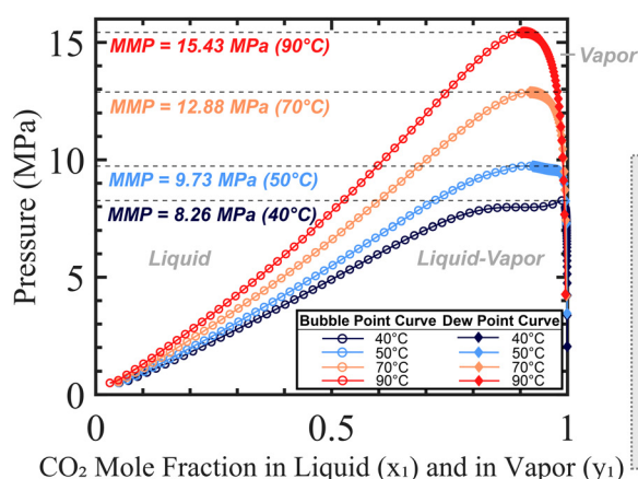
Fig. 9 Prediction of the minimum miscibility pressure (MMP) using the Peng–Robinson equation of state (PR-EOS). (A) Phase envelopes of CO 2 /n-decane mixtures at T = 40, 50, 70 , and 90\text{ }^{\circ}\text{C} , computed using PR-EOS. The phase envelope consists of the bubble point curve (open \circ ), which plots the bubble point pressure P_{\text{bubble}} against the CO 2 mole fraction in the liquid phase ( x_1 ), and the dew point curve (filled \bullet ), which plots the dew point pressure P_{\text{dew}} against the CO 2 mole fraction in the vapor phase ( y_1 ). MMP is determined at the highest point of P on the phase envelope, above which the two components form a fully miscible, single-phase mixture at all proportions. (B) Flow chart illustrating the bubble point calculation procedure. CO 2 is treated as component 1 and n -decane as component 2. For each specific CO 2 liquid mole fraction x_1 , the corresponding bubble point pressure P_{\text{bubble}} and vapor mole fraction y_1 are obtained using a Newton–Raphson method based on PR-EOS with the van der Waals mixing rule. The iteration converges when the fugacity residual between liquid and vapor phases, \|F = f_L - f_V\| , falls below a tolerance of 10^{-6} , satisfying vapor–liquid equilibrium (VLE). By the same token, dew point pressures ( P_{\text{dew}} ) are calculated analogously by fixing y_1 and solving for x_1 and P_{\text{dew}} . Each converged solution contributes to the construction of the phase envelopes in Fig. 9A.
