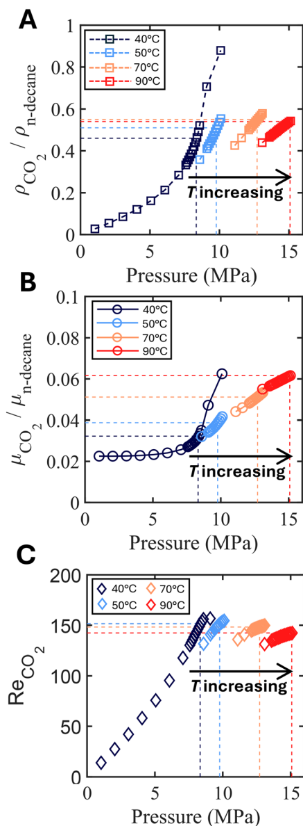
Fig. 12 Variation of dimensionless parameters at different temperatures and pressures. (A) The density ratio \rho_{\text{CO}_2}/\rho_{\text{n-decane}} , (B) the viscosity ratio \mu_{\text{CO}_2}/\mu_{\text{n-decane}} , and (C) the Reynolds number of \text{CO}_2 .
