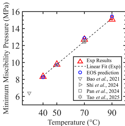
Fig. 10 Comparison of minimum miscibility pressure (MMP) determined from our microfluidic experiments using dynamic flow ( \Delta ) and Peng-Robinson EOS predictions ( \circ ) at T = 40, 50, 70 , and 90 °C. Literature data using dead-end microfluidic channels to determine \text{CO}_2 -decane MMP from Bao et al. 75 ( \nabla ), Shi et al. 76 ( \triangleright ), Pan et al. 77 ( \square ) and Tao et al. 78 ( \star ). Error bars represent the scatter across three independent experimental datasets, calculated as 0.5 \times (\text{MAX} - \text{MIN}) . A linear regression of the experimental data is shown as a dashed line, given by \text{MMP (MPa)} = 0.136 \times T (\text{°C}) + 2.976 , with a coefficient of determination R^2 = 0.997 .
