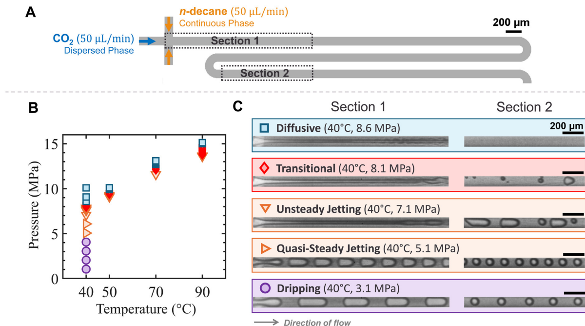
Fig. 2 (A) Microchannel schematic showing section 1 and section 2 as the regions of interest under a microscope with a 10× objective. CO 2 (dispersed phase) and n -decane (continuous phase) were co-injected at a constant flow rate of 50 μL min -1 at the flow-focusing junction. Section 1 captures the junction where the CO 2 -decane interface forms, while section 2 is located downstream (8.6 mm from the junction). (B) Phase diagram summarizing all the experimental conditions, showing flow regime transitions at T = 40, 50, 70, and 90 °C. (C) Representative snapshots at T = 40 °C for each flow regime, captured from section 1 (left) and section 2 (right) as indicated in (A). Experimental conditions are noted; scale bars: 200 μm.
