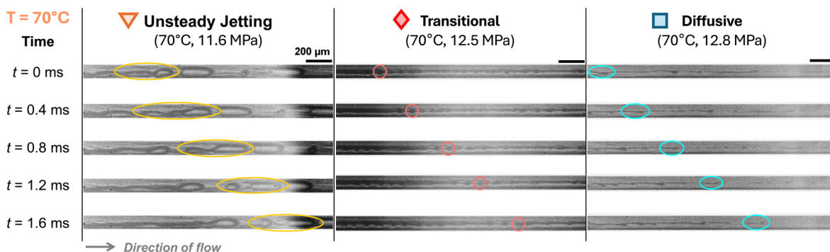
Fig. 6 Time-lapse snapshots at T = 70\text{ }^{\circ}\text{C} showing the evolution of the CO 2 jet tip at 11.6 MPa (unsteady jetting), 12.5 MPa (transitional), and 12.8 MPa (diffusive). Scale bars: 200 μm.
