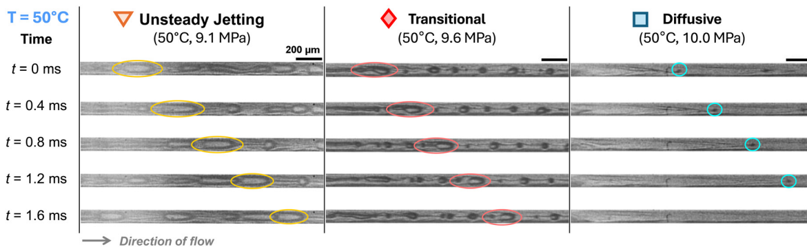
Fig. 5 Time-lapse snapshots at T = 50\text{ }^{\circ}\text{C} showing the evolution of the CO 2 jet tip at 9.1 MPa (unsteady jetting), 9.6 MPa (transitional), and 10.0 MPa (diffusive). Scale bars: 200 μm.
