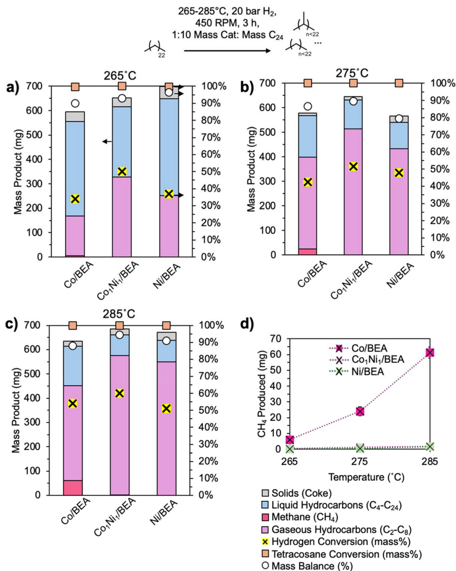
Fig. 7 Temperature-dependent hydrocracking performance. (a–c) Product distribution (methane, C 2 –C 8 gas, C 4 –C 24 liquid, solid) from tetracosane hydrocracking at 265 °C, 275 °C, and 285 °C over Co/BEA, Ni/BEA, and Co 1 Ni 1 /BEA (700 mg substrate, 70 mg catalyst, 3 h reaction). (d) Methane yield as a function of temperature for all catalysts. Detailed product distributions are provided in the SI.
