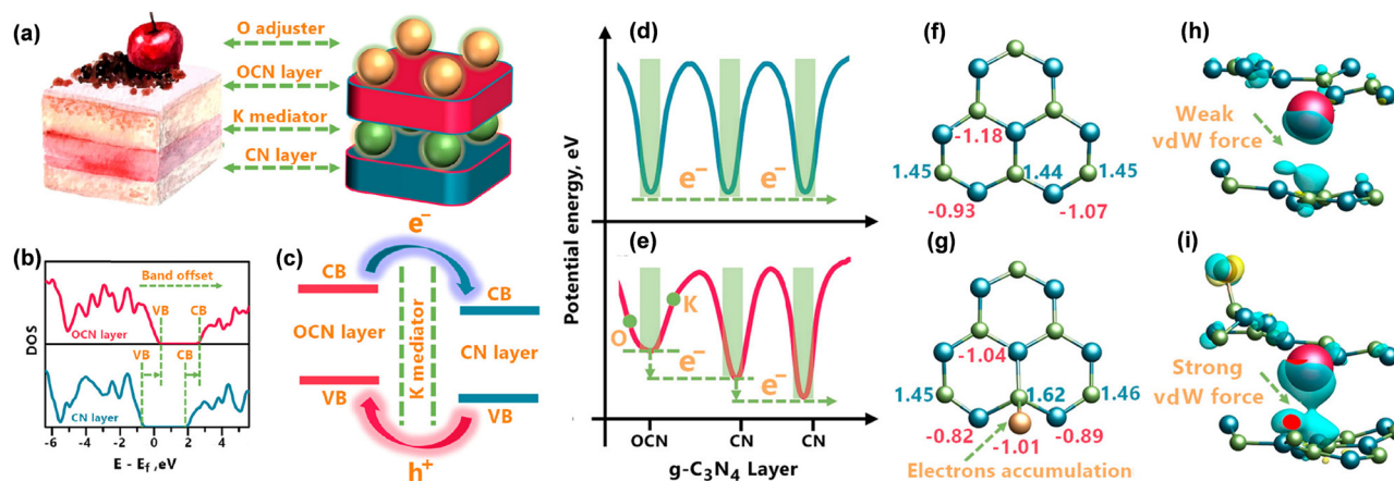
Fig. 30 (a) Schematic representation of the internal van der Waals (VDWH) and structural framework of OCN-K-CN, (b) calculated total density of states (TDOS), (c) band alignment diagram of the OCN-K-CN IVDWH, (d) and (e) layered electrostatic potential distribution, (f) and (g) Bader charge distribution for pristine CN and OCN-K-CN, (h) and (i) charge density difference mapping of K-CN and OCN-K-CN, where blue, green, red, and gold spheres correspond to N, C, K, and O atoms, respectively. Reproduced with permission from ref. 190. Copyright 2018, American Chemical Society.
