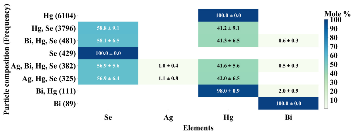
Fig. 7 Heatmap of the detected particles containing Se, Ag, Hg or Bi (or a combination thereof). Particle numbers in parentheses refer to a sample that was diluted 100× (9 minutes analysis time, transport efficiency = 0.383 \mu\text{L s}^{-1} ). The annotation on the heatmap gives the average molar percent ( \pm standard deviations) for each element in the particle. Particles were extracted from ~20 mg of a bearded seal liver using 5 mL of formic acid.
