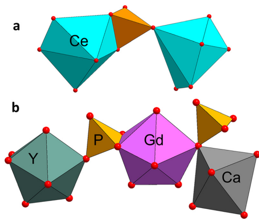
Fig. 7 Coordination of the CeO 7 (a) and GdO 8 (b) polyhedra in CFA. Ce, cyan; Gd, purple; Y, light green; P, light brown; O, red.
