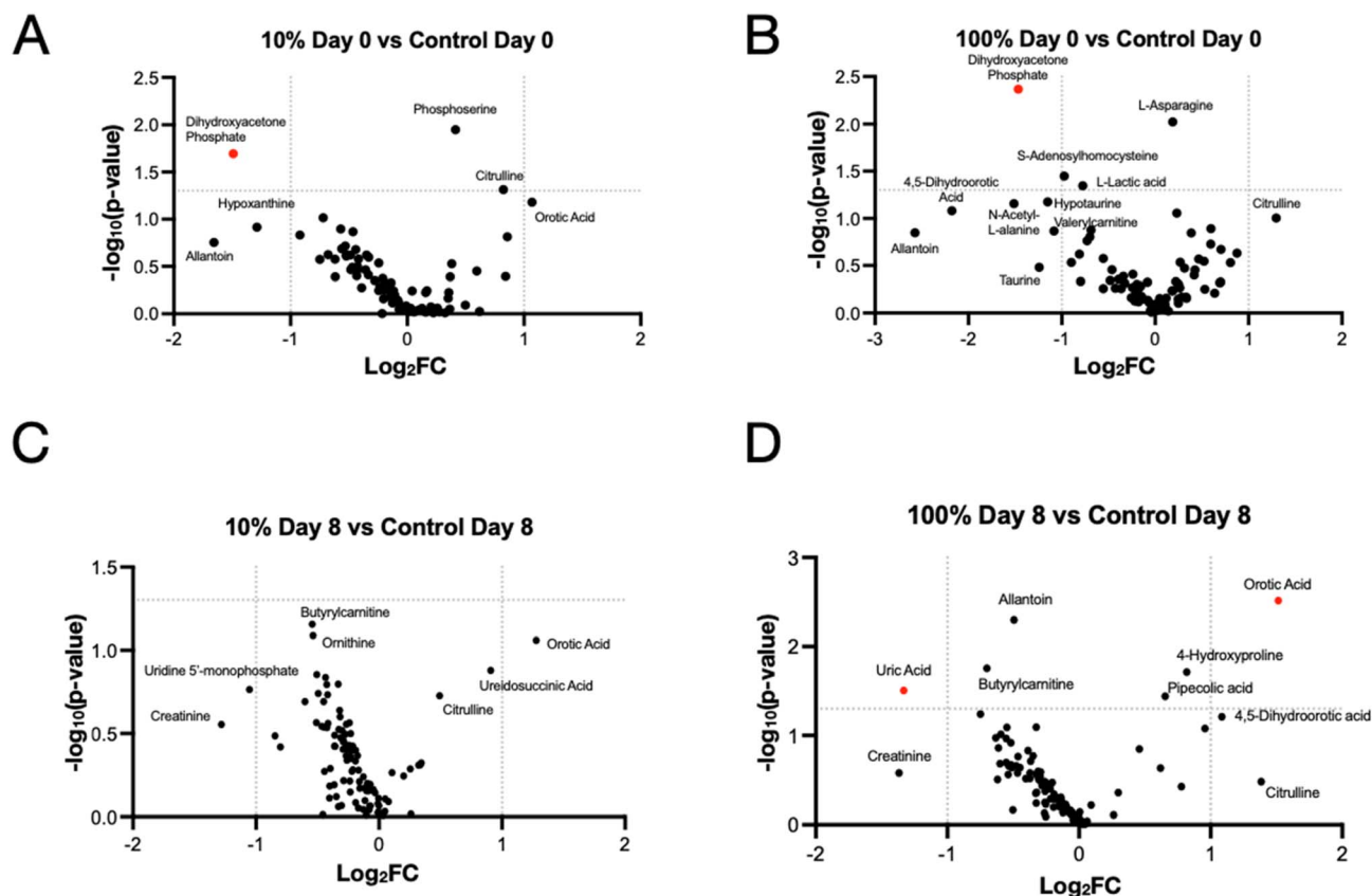
Fig. 4 The magnitude of metabolomic changes in worms exposed to sodium arsenite is small. Volcano plots ( -\log_{10}(p\text{-value}) vs. \log_2FC ) of metabolites identified in (A) 10% LC 10 day 0 vs. control day 0, (B) 100% LC 10 day 0 vs. control day 0, (C) 10% LC 10 day 8 vs. control day 8, and (D) 100% LC 10 day 8 vs. control day 8.
