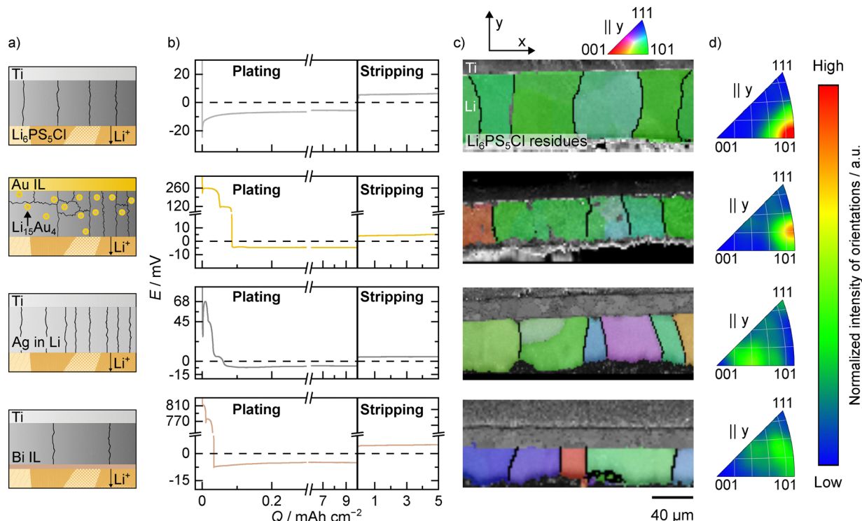
Fig. 4 Microstructure of electrodeposited lithium after partial stripping. (a) Cell setup used for stripping after electrodeposition of 10 mAh cm -2 of lithium. The location of the interlayers is indicated schematically. (b) Potential profile during electrodeposition of 10 mAh cm -2 lithium on the left and subsequent stripping of 5 mAh cm -2 on the right. (c) Microstructure of the partially stripped lithium layers using the different interlayer materials. The IPF maps are given parallel to the y-direction as indicated above. The shown scalebar resembles 40 μm in all cases. (d) IPFs of the partially stripped lithium layers, showing the distribution of all measured grain orientations. Please note that the IPFs were created based on the entire analyzed cross-section, which is shown in the SI.
