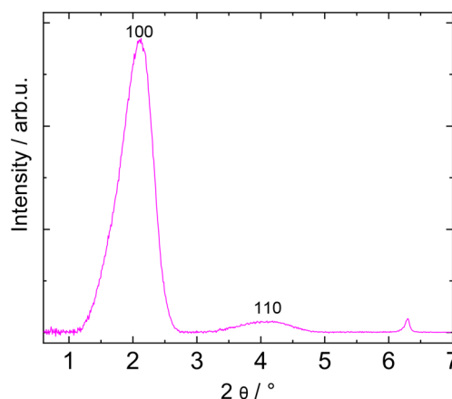
Fig. 3 Exemplary small angle XRD pattern for the completely transformed material C18.
