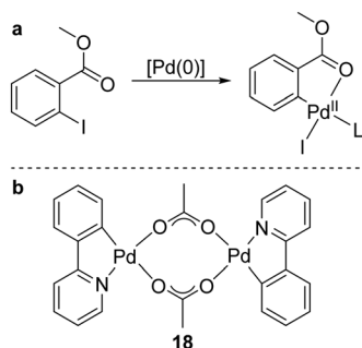
Scheme 5 a) Proposed ortho -coordination between methyl 2-iodobenzoate and palladium following oxidative addition, and prior to isomerisation. Pd speciation in the DES is likely to be complex. There are many species capable of coordinating at position L (e.g. [OAc] − , Cl − , I − , urea, H 2 O, [Ch] + ). b) Palladacycle 18 prepared to explore metallocycle reactivity.
