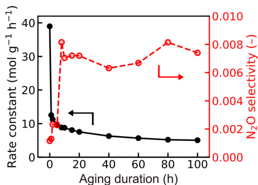
Fig. 2 Rate constants (mol g -1 h -1 ) for NO conversion and N 2 O selectivity as a function of hydrothermal aging duration at 650 °C for 3.2 wt% Cu-CHA (an SAR of 13.4). Measurements were performed using 50 mg of catalyst exposed to a gas mixture containing 500 ppm NO, 600 ppm NH 3 , 10% O 2 , and 5% H 2 O, at 160 °C in an N 2 carrier gas with a total flow rate of 13.5 NL h -1 .
