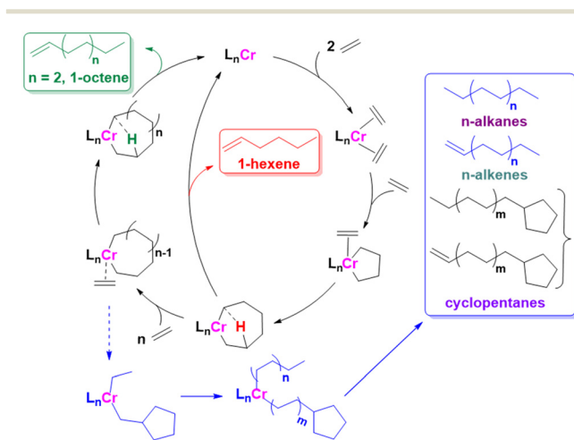
Scheme 1 Ethylene oligomerization via the metallacyclic mechanism. 3,10,11
