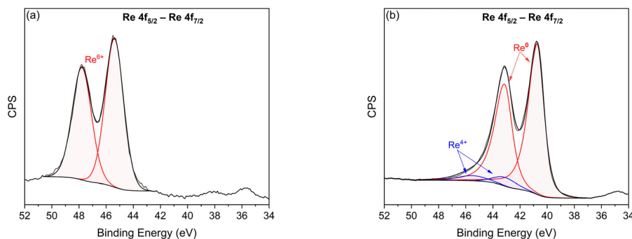
Fig. 3 In situ XPS of (a) the Re 4f region for the \text{ReO}_x/\text{G} catalyst and (b) the Re 4f region for the \text{Re}/\text{G} catalyst.
