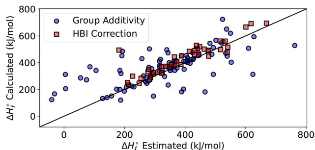
Fig. 5 Standard enthalpies of formation ( \Delta_f H_{298\text{K}}^\circ ) calculated at DLPNO-CCSD(T)-F12/cc-pVTZ-F12// \omega B97X-D/def2-TZVP are compared to estimates by RMG, 15,16 including group additivity (blue circles) and HBI corrections 48 (red squares).
