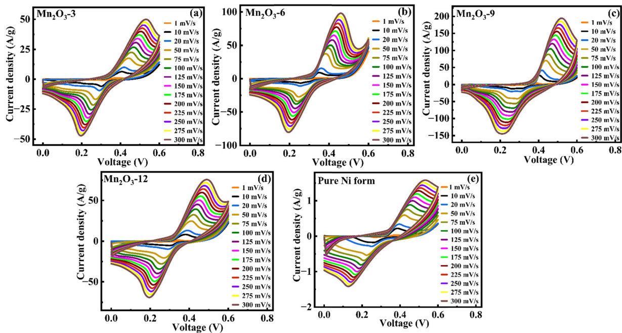
Fig. 6 Cyclic voltammograms of (a)–(d) \text{Mn}_2\text{O}_3\text{-}x and (e) pure Ni form at different scan rates from 1–300 \text{mV s}^{-1} in 1 M KOH electrolyte.
