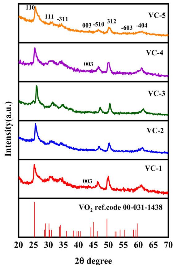
Fig. 1 pXRD pattern of the VO 2 /carbon composites (VC-1 to VC-5).
