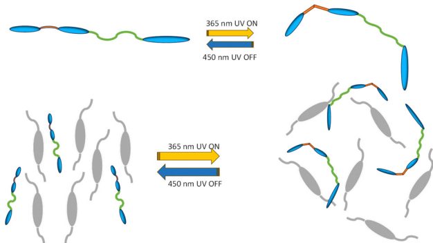
Fig. 17 Picture depicting the situation where spacer length is fixed at n = 6 .
