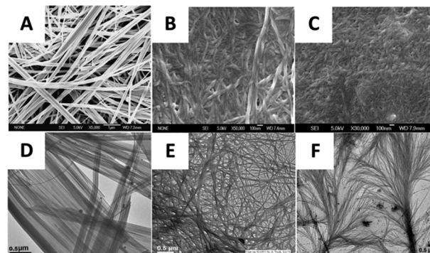
Fig. 8 Self-assembling branched peptide organogels. Three different generations of branched peptides were compared, each undergoing the coupling of an additional generation of amino acids. (A)–(C) Field emission scanning electron micrographs of the resulting gels at the three different generations. (A) Shows the fewest number of generations and least dense network, whilst (B) is the median number of generations and density, and (C) is the largest number of generations forming the densest network. (D)–(F) High-resolution transmission electron micrographs (HR-TEM) of the branched gels obtained from the different generations of dendritic 1,2-dichlorobenzene. Reproduced with permission from ref. 162 Copyright 2024, American Chemical Society.
