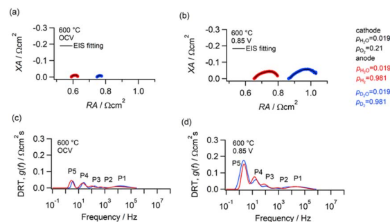
Fig. 4 Nyquist plots and DRT spectra of PCFCs at 600 °C when the gas at the anode is replaced by light hydrogen to heavy hydrogen. Impedance spectra under (a) OCV and (b) polarization states (0.85 V). DRT spectra under (c) OCV and (d) polarization states (0.85 V).
