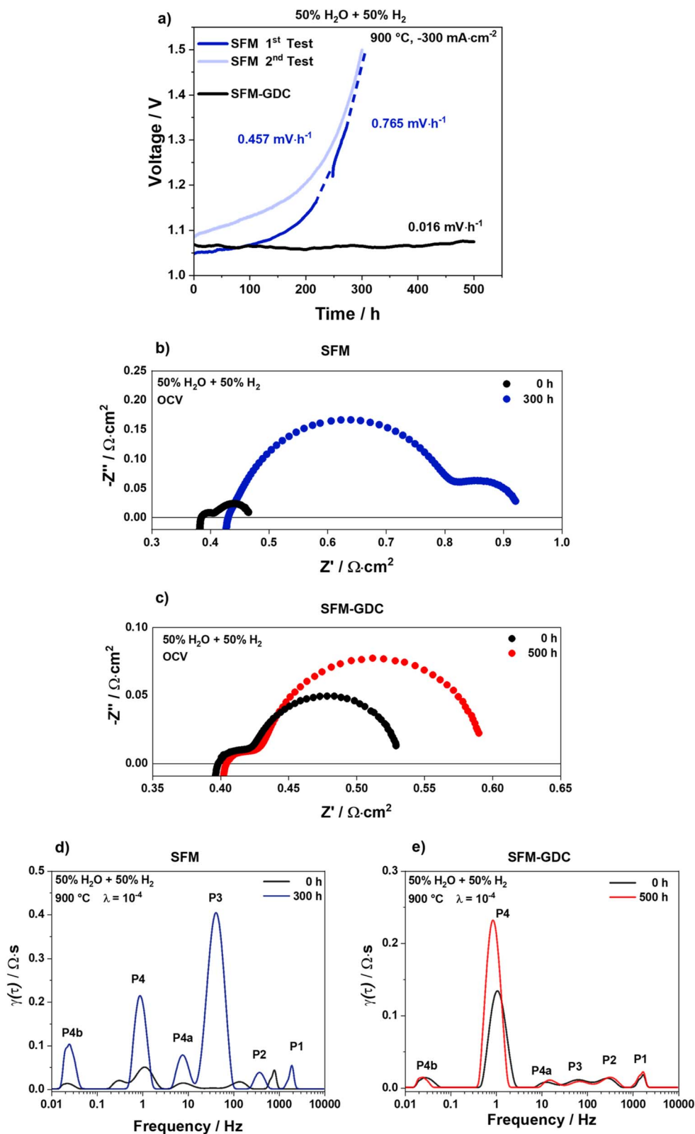
Fig. 8 (a) Long-term stability test of single cells with SFM/GDC/8YSZ/GDC/LSCF and the composite SFM-GDC/GDC/8YSZ/GDC/LSCF in 50% H 2 O + 50% H 2 fuel gas composition under constant -0.3 A cm -2 current load at 900 °C for up to 500 h. Comparison of (b and c) the Nyquist plots and (d and e) the corresponding DRT spectra recorded before and after the durability test.
