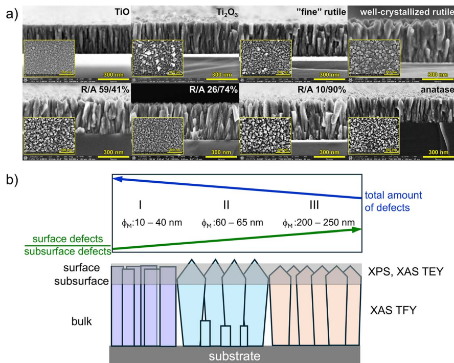
Fig. 10 Scanning electron microscopy cross-sectional images and top views of titanium oxide thin films obtained via reactive RF magnetron sputtering (a). Schematic representation of three different classes of Ti–O photoanodes (b).
