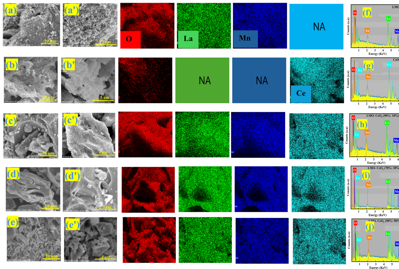
Fig. 3 FESEM images at 20 μm and 5 μm magnifications for (a and a') LMO, (b and b') CeO 2 , (c and c') LMO–CeO 2 (90% : 10%), (d and d') LMO–CeO 2 (70% : 30%), and (e and e') LMO–CeO 2 (50% : 50%). Elemental mapping of O (red), Mn (blue), La (green), and Ce (cyan color) at 5 μm highlights the distribution of elements in different LaMnO 3 –CeO 2 composites. (NA: not applicable.)
