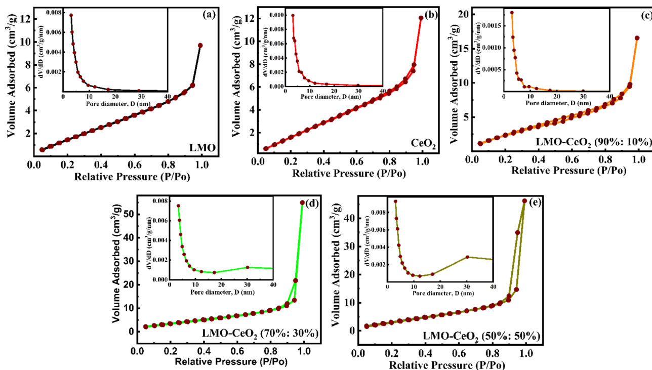
Fig. 4 (a–e) Nitrogen adsorption–desorption isotherms of LMO–CeO 2 composites, with corresponding BJH pore size distribution curves shown in the inset.
